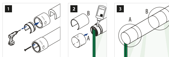
Q-49 Q-20 Q-21 Q-glu, 50 ml 19.1331.000.00
