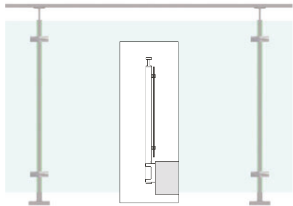
96 Glass clamps - MOD 29
