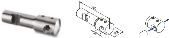
Quickrail® - bar
