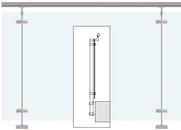
96 Glass clamps - MOD 29
