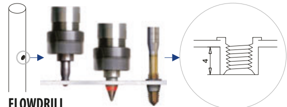
FLOWDRILL
